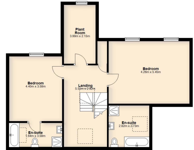
Third Floor Approx. 80.7 sq. metres
